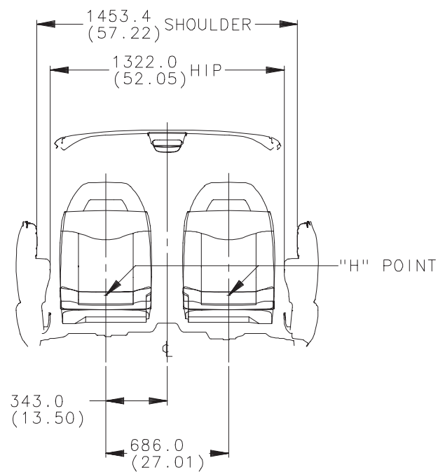
FRONT VIEW OF FRONT SEAT
