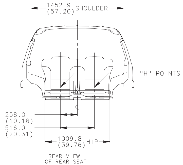
REAR VIEW OF REAR SEAT
