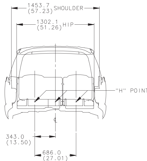
REAR VIEW OF REAR SEAT
