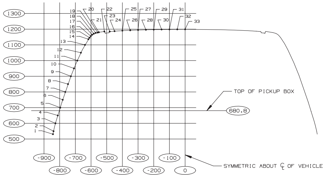
SECTION B-B
