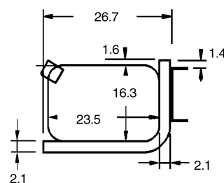
Side View Fuel Tank
