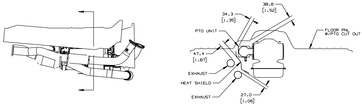
CHELSEA P.T.O. MOUNTED TO M74 AUTOMATIC TRANSMISSION
