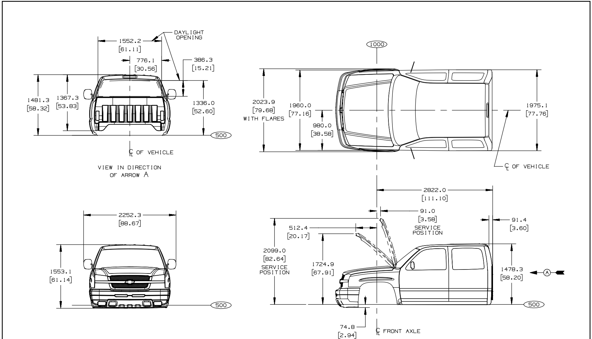
C/K (25HD/35/36) CREW CAB EXTERIOR (CHEVY)
