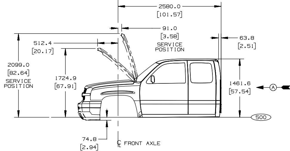
C/K (25HD/35/36) EXTENDED CAB EXTERIOR (CHEVY)
