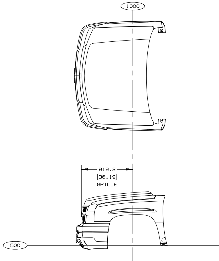
HOOD & GRILLE C/K (25HD/35/36) (03/43/53), 2005 X88 MID-CYCLE ENHANCMENT
