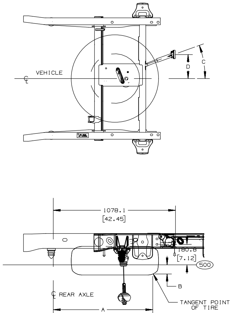
C/K (15/25) SPARE TIRE PICKUP 2003/04
