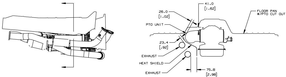
MUNCIE P.T.O. MOUNTED TO M74 AUTOMATIC TRANSMISSION
