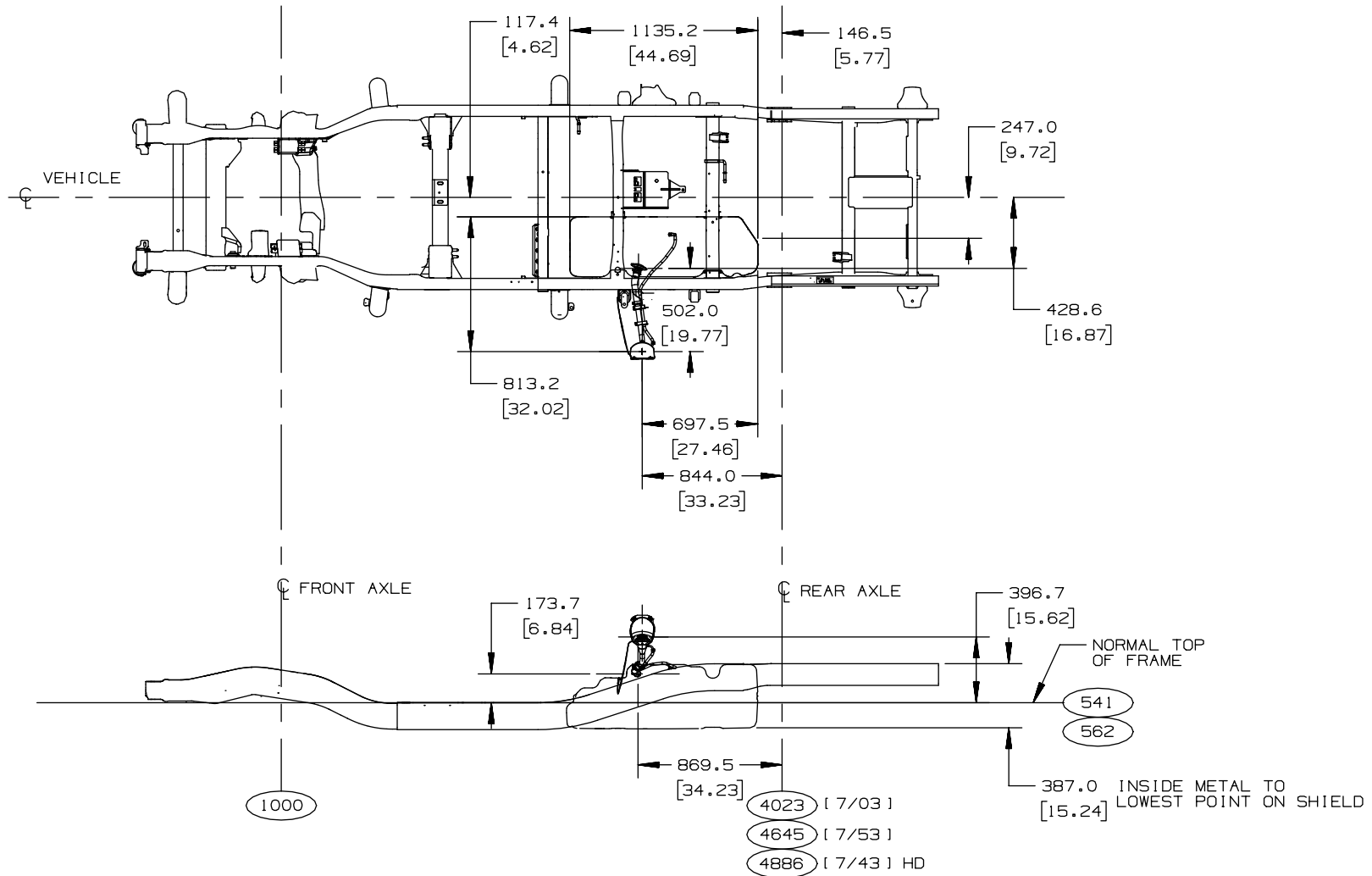
C/K (15/25) (7) (03/43/53) 26 GALLON FUEL TANK
