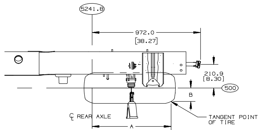
C/K (25HD/35) SPARE TIRE CARRIER 2003
