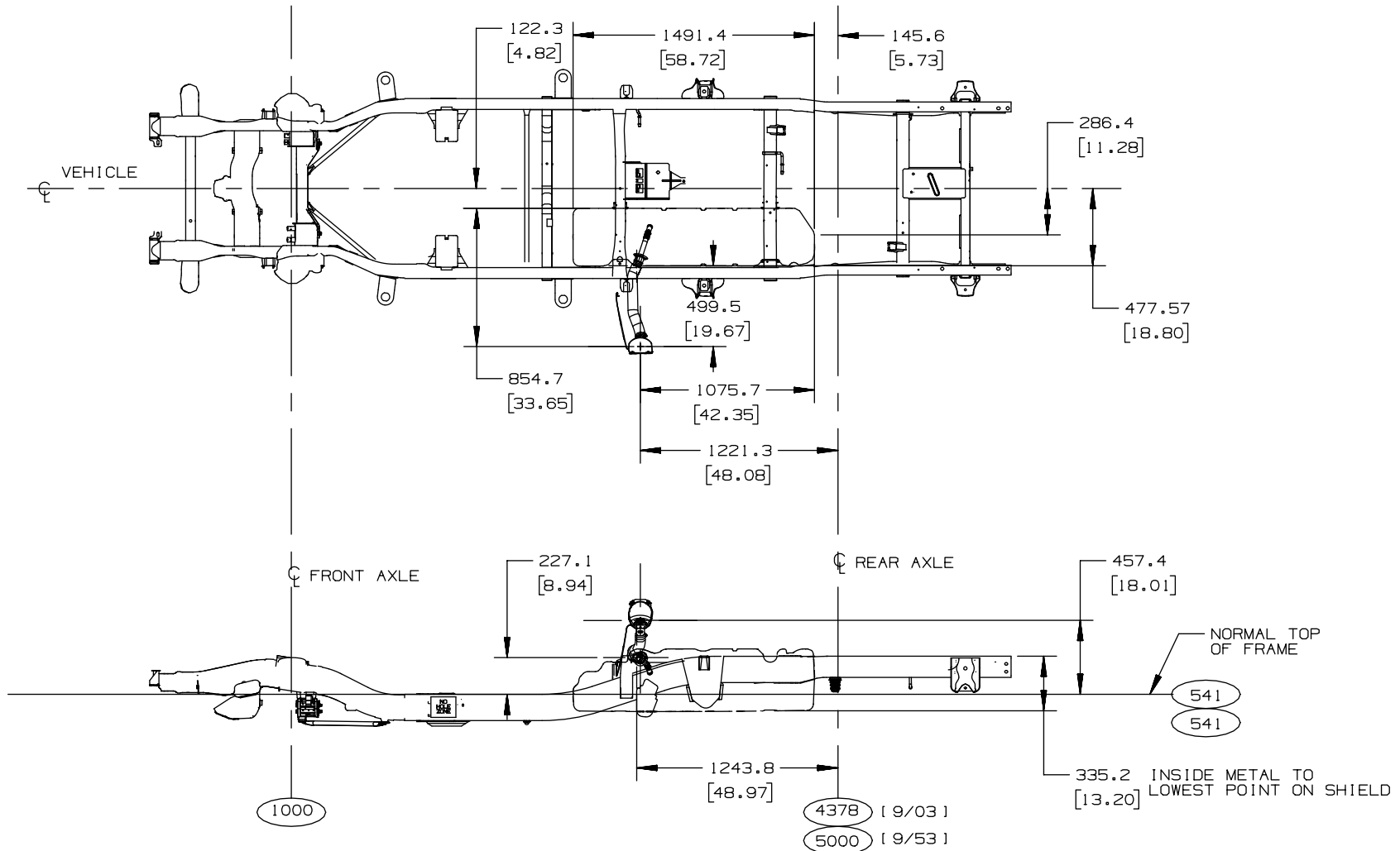
C/K (15/25)(9)(03/53) 34 GALLON FUEL TANK
