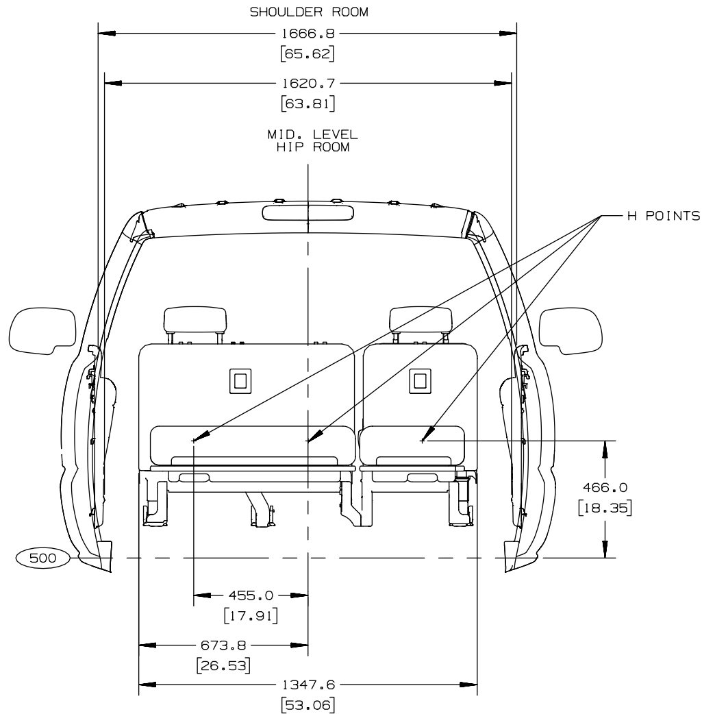
REAR VIEW SHOWING REAR SEATS FOR CREW CAB
