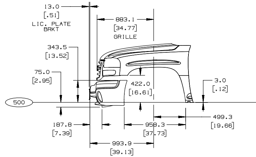
C/K (25HD/35/36) FRONT END SHEET METAL
