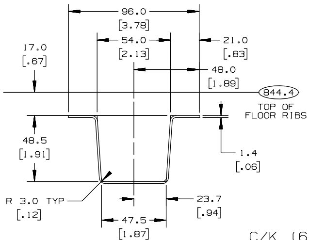
SECTION B-B TYPICAL 3 PLACES
