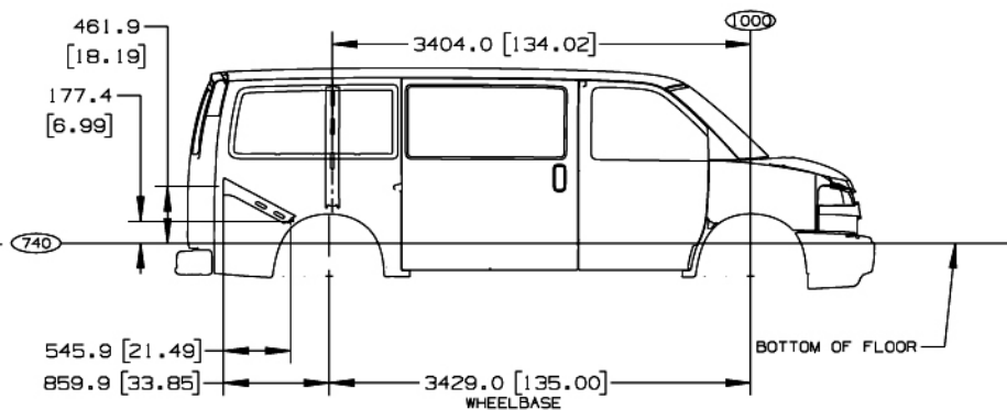
R.H. SIDE VIEW (YA2)
