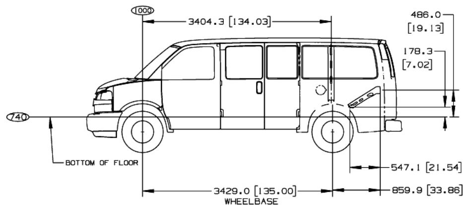
L.H. SIDE VIEW (E26)
