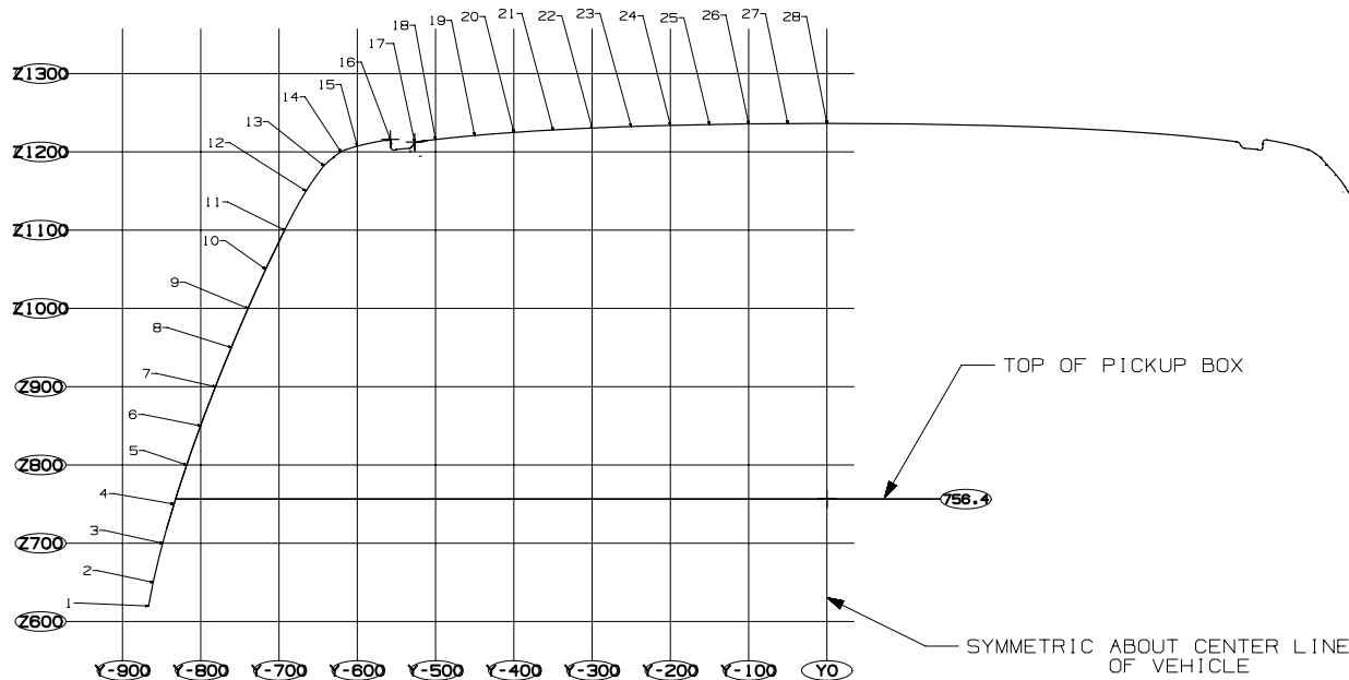
SECTION B-B
