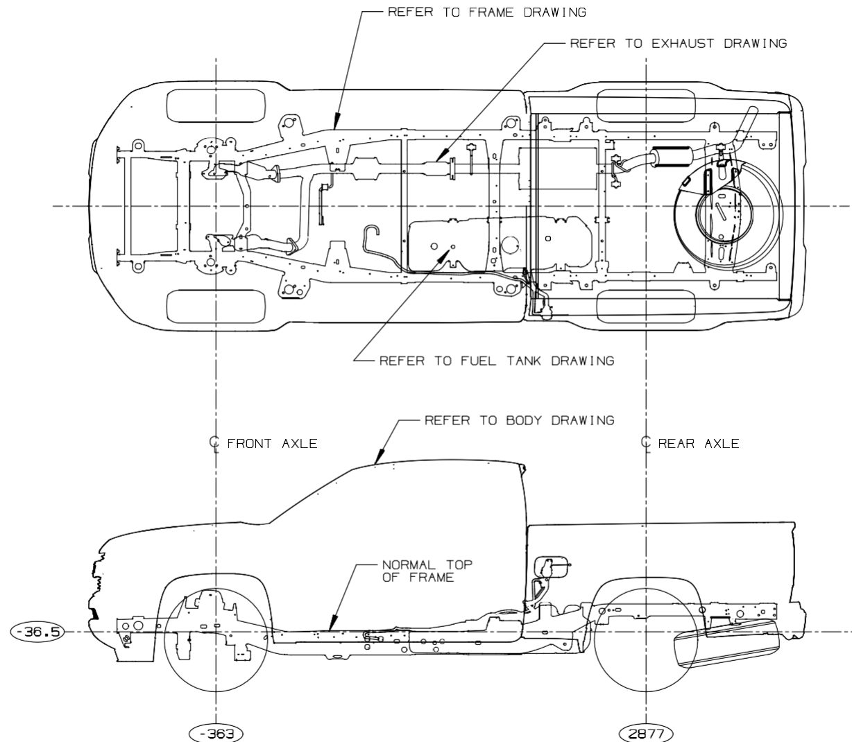
1/T2M53 (SWB P/U Ext. Cab) General Arrangement
