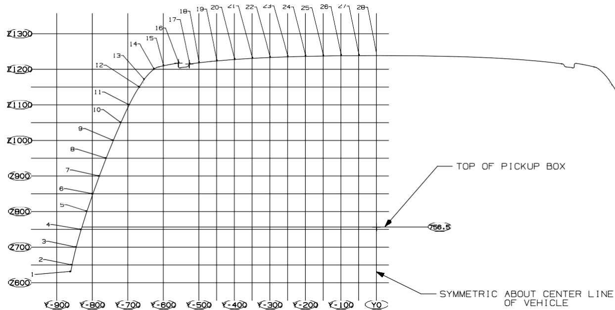
SECTION C-C
