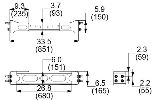
3 PIECE CROSSMEMBER
