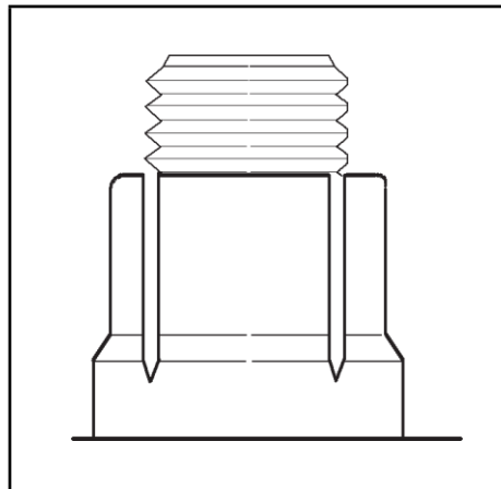
Figure-01-17 Collar with Reliefs for Removal 01_0027
