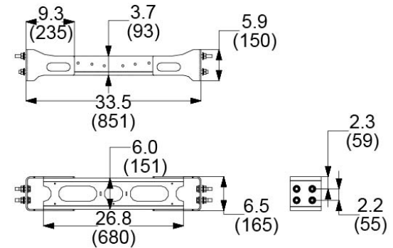
3 PIECE CROSSMEMBER
