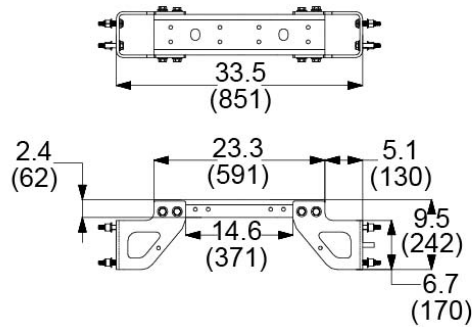
REAR CAB MOUNTING CROSSMEMBER
