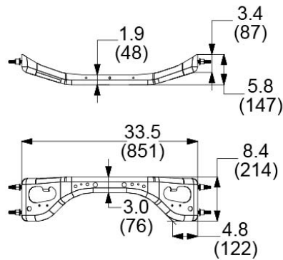
SINGLE DOGBONE CROSSMEMBER
