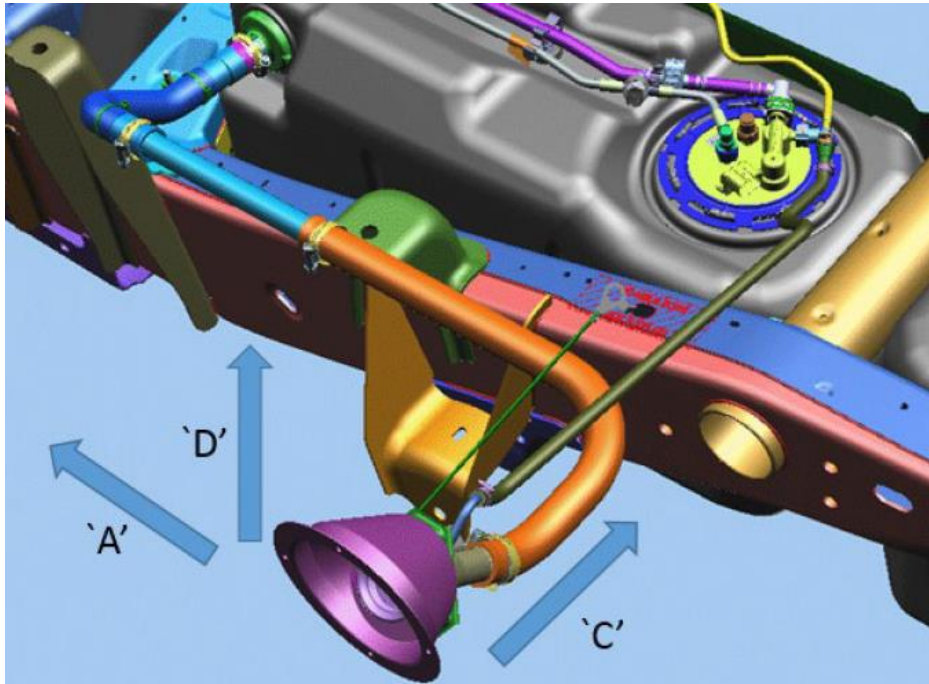
84709155 HD Pickup ZW9 `GAS'(FJW) Fuel Fill Assembly (above)
