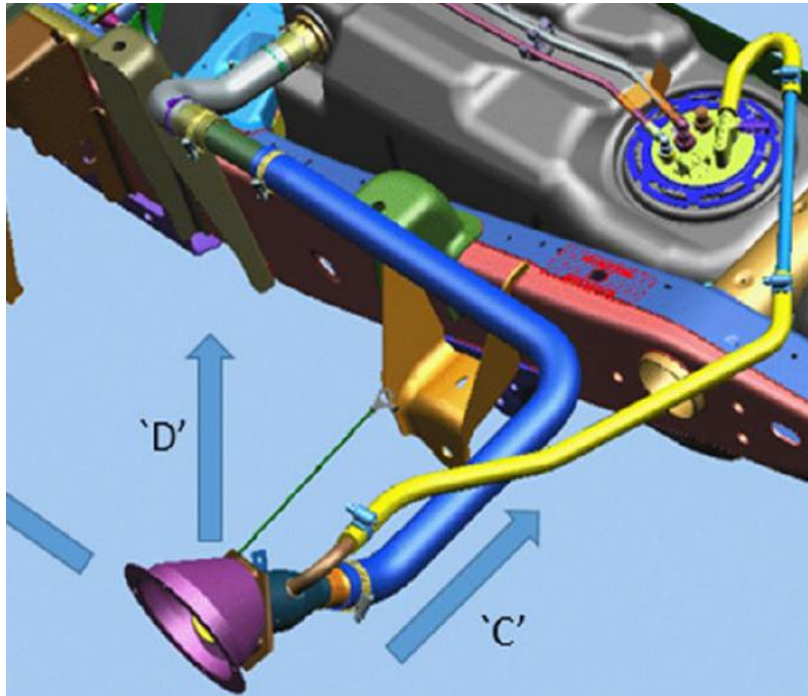
84861894 HD Pickup ZW9 `DIESEL'(FHX) Fuel Fill Assembly (above)
