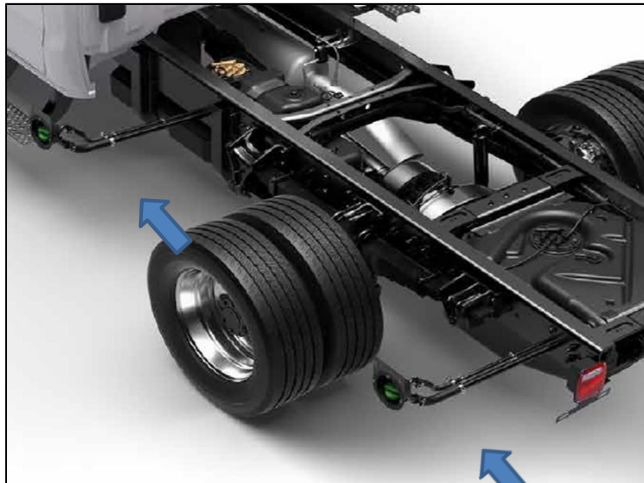
Figure 3 – Factory Equipped Straight Fill Hose Assembly
