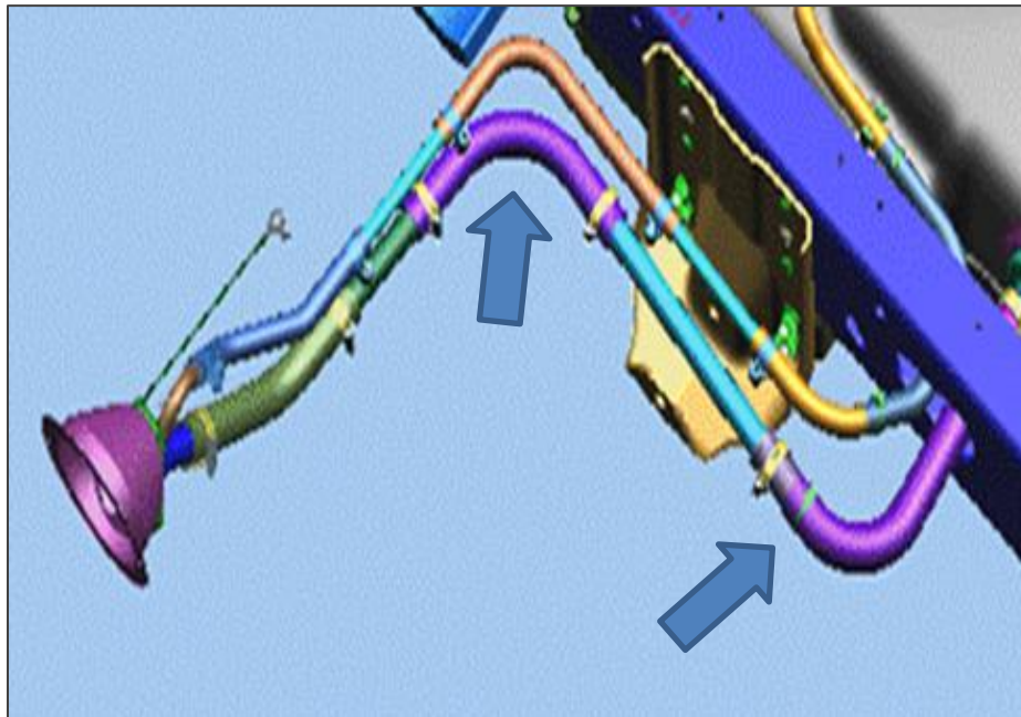
Figure 4 - Fuel Filler with Elbow Kit (Purple) installed by Upfitter
