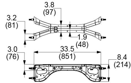
DOUBLE DOGBONE CROSSMEMBER
