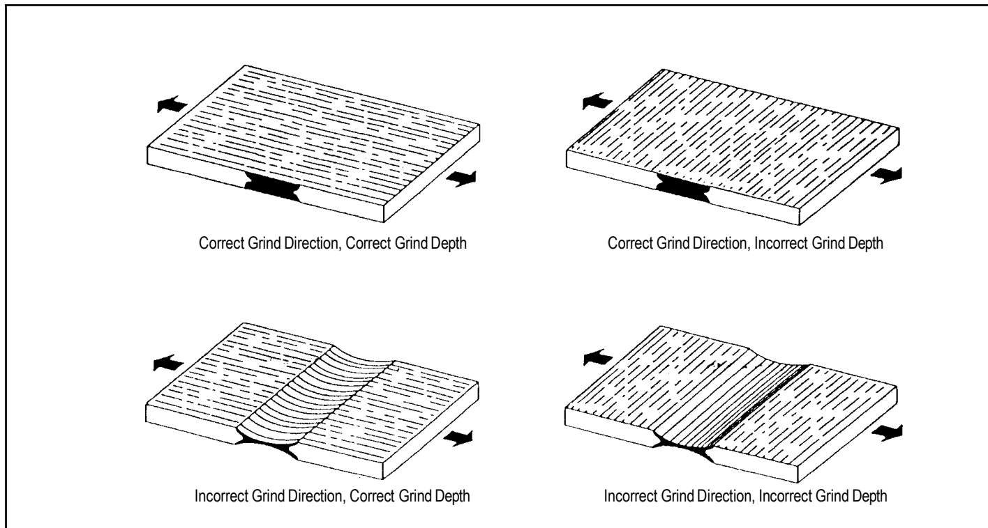
Figure-01-25 Cross-sectional Views Showing Correct and Incorrect Methods of Finishing the Joint
