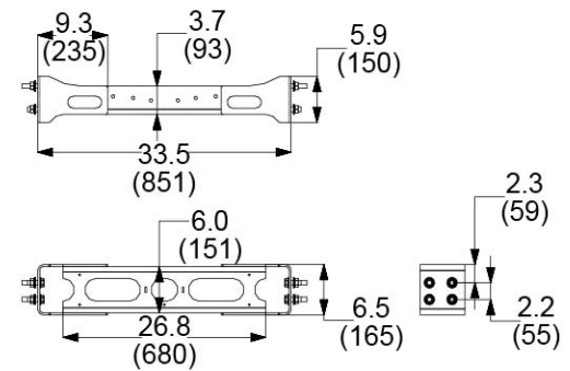
3 PIECE CROSSMEMBER
