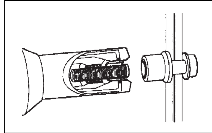
Figure-01-12 Body of Fastener Separates at Breakneck
