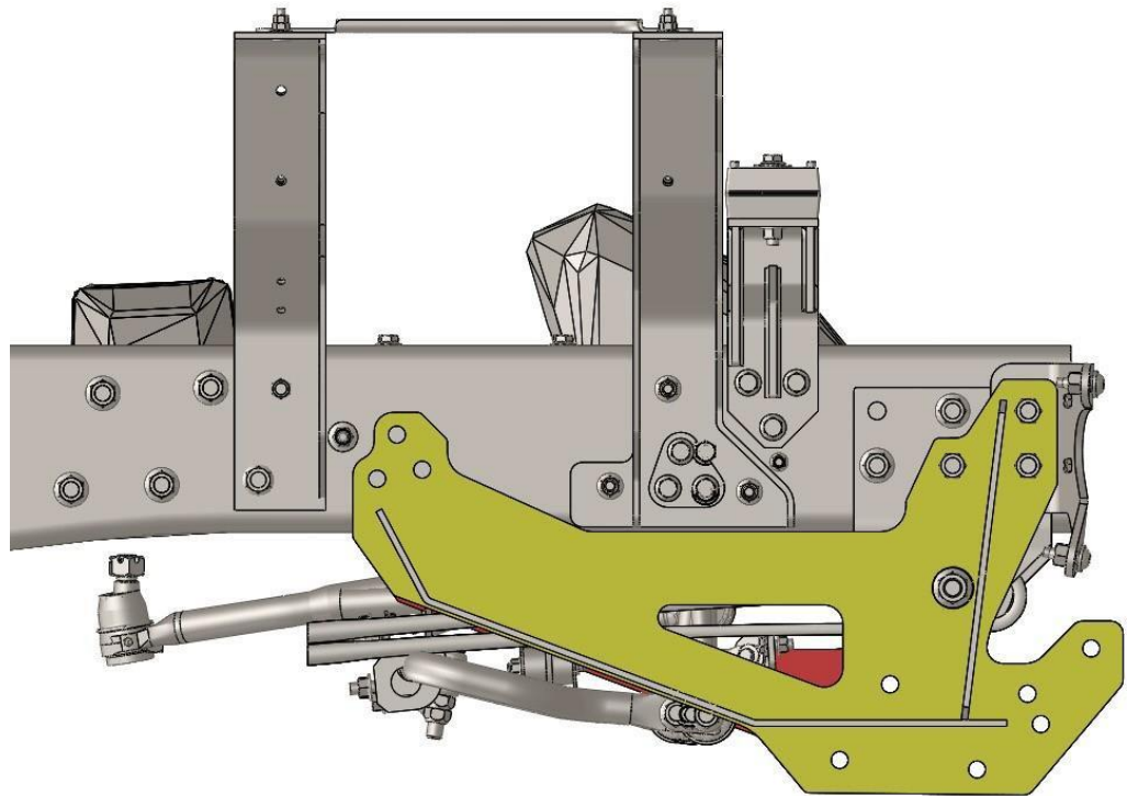
Suggested Snow Plow Attachment
