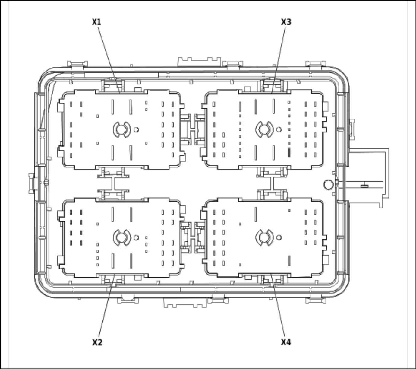
X50A Engine Wiring Harness Junction Block Bottom View
