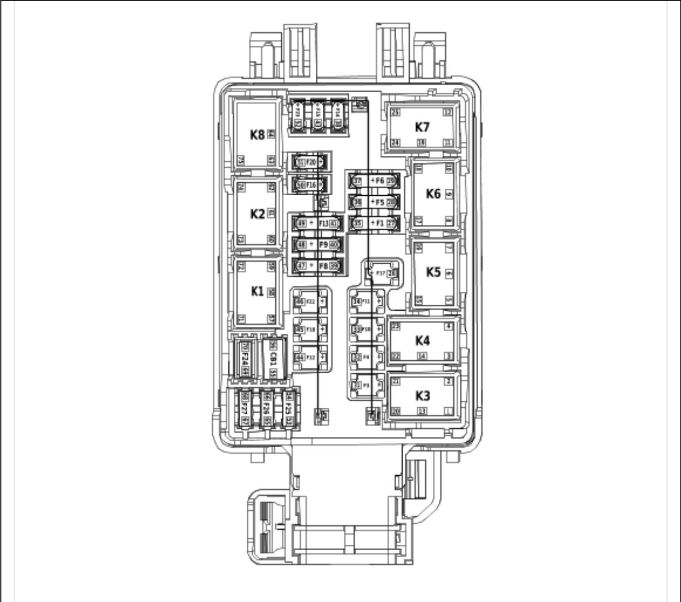
X53AF Body Wiring Harness Junction Block Top View
