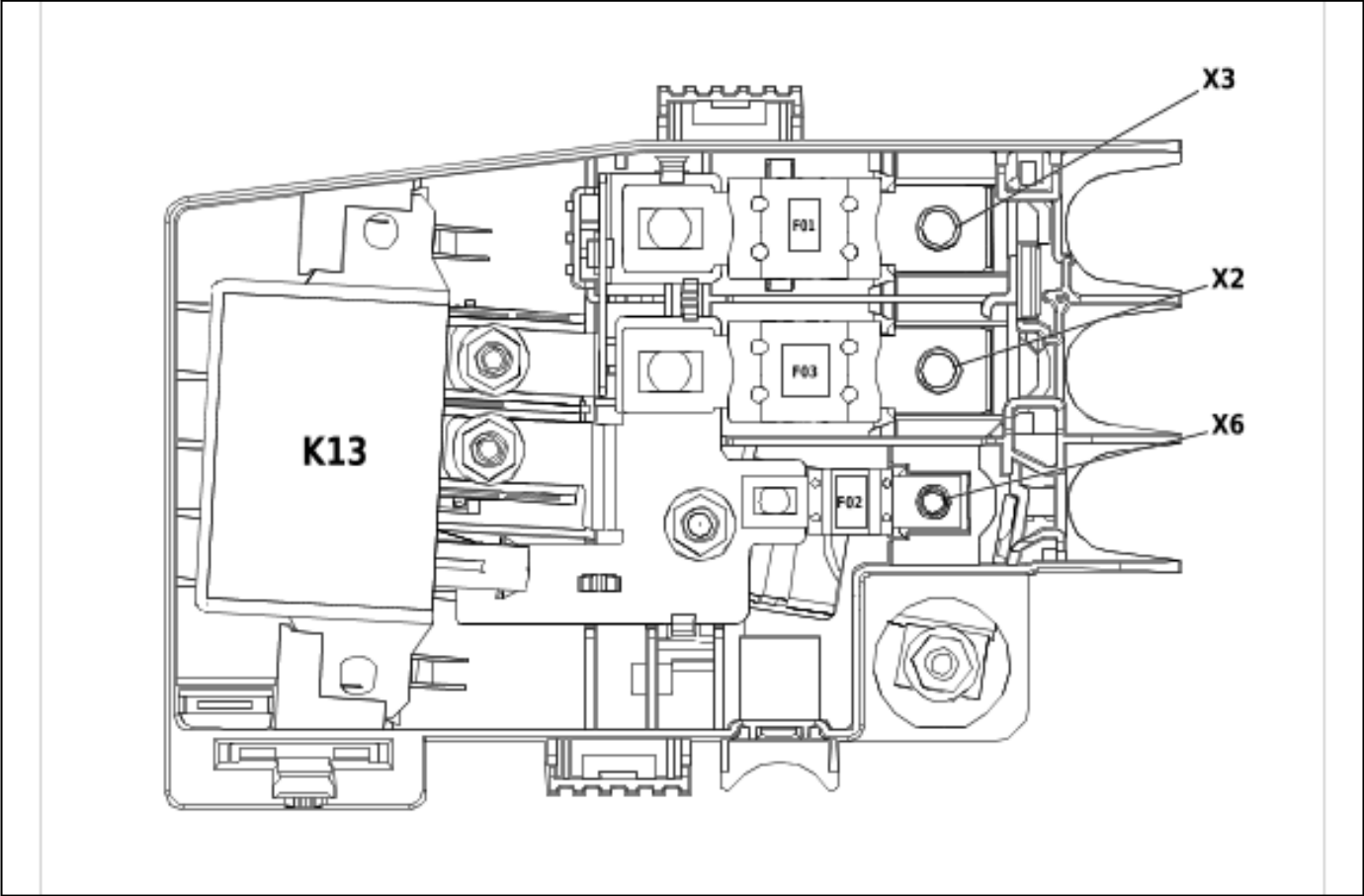
X50EA Battery Distribution Fuse Block - Auxiliary Top View (L8T & K4Z)
