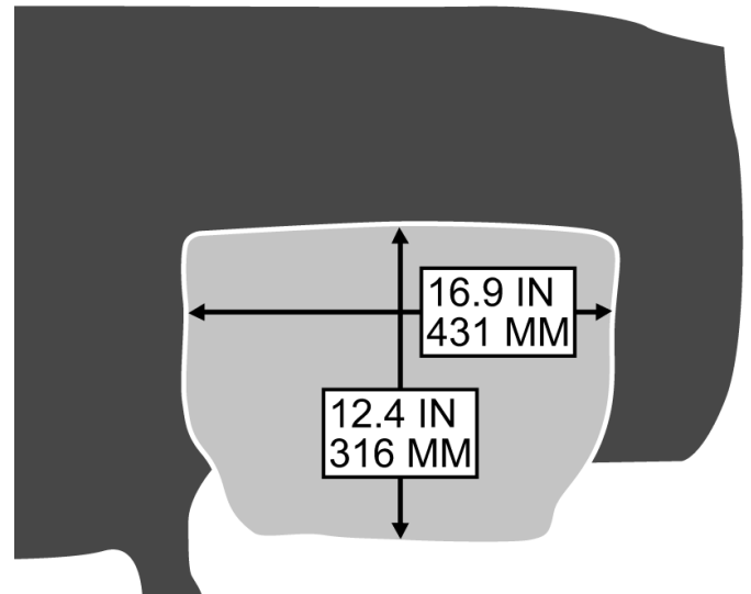
KNEE AIRBAG FRONT VIEW FROM PASSENGER SIDE
