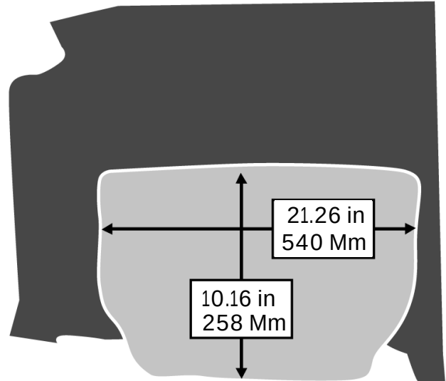
KNEE AIRBAG FRONT VIEW FROM DRIVER SIDE
