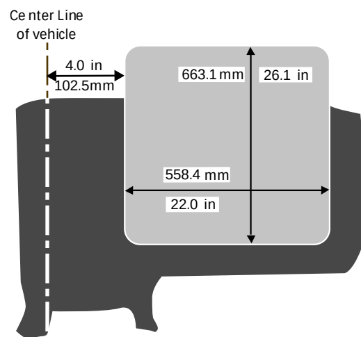
FRONT OUTBOARD PASSENGER AIRBAG VIEW FROM PASSENGER SIDE
